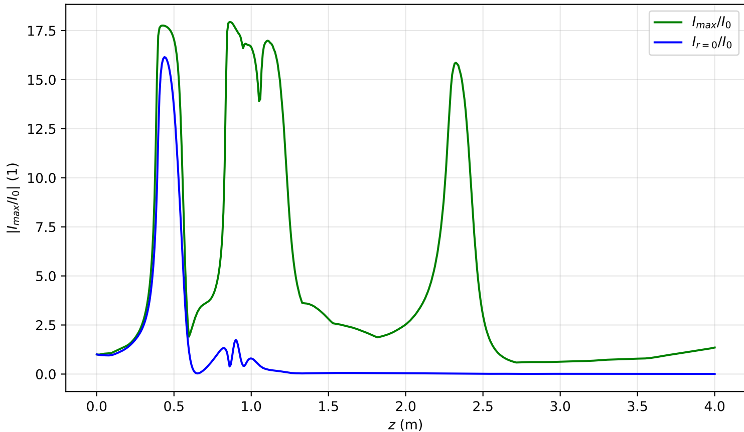
I_{max}(x = 0, y = 0, z)/I_0 , P_{in}=6.2P_{cr} , noisy input, artificial time
